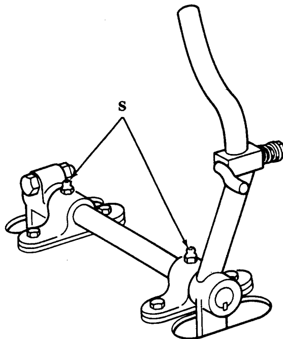
DUMP LEVER CROSS-SHAFT
