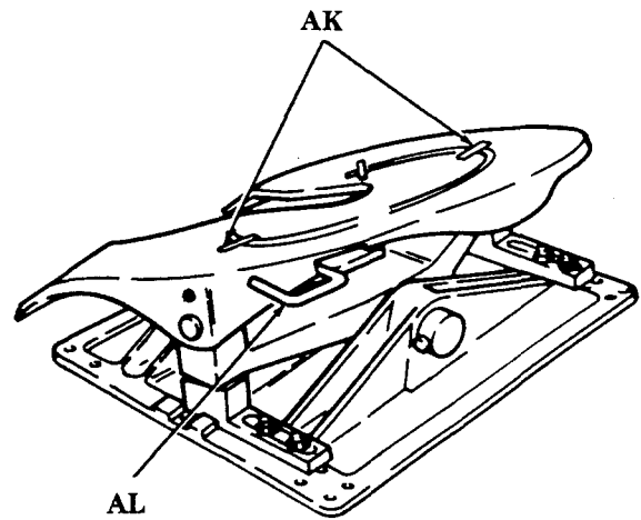
FIFTH WHEEL
