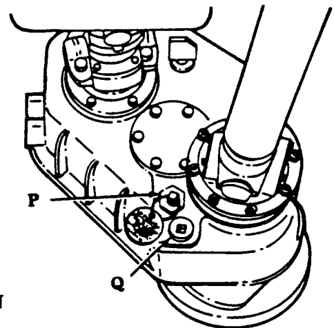
TRANSFER CASE
