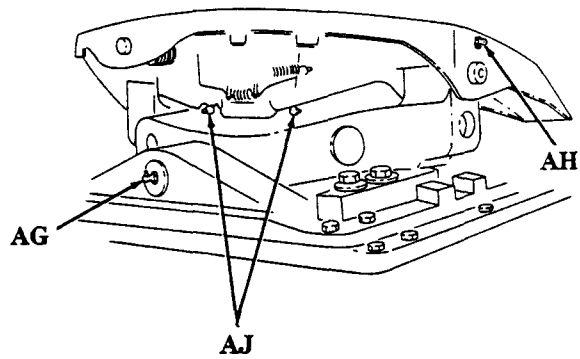
FIFTH WHEEL
