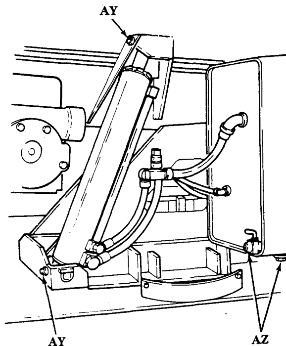
WRECKER ELEVATING CYLINDER
