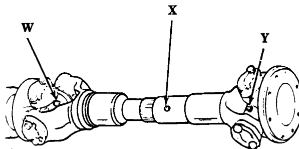
UNIVERSAL AND SLIP JOINT
