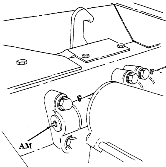
TRUNNION PIN
